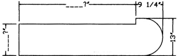
13" BULLNOSE STARTING STEP (RIGHT HAND SHOWN)
