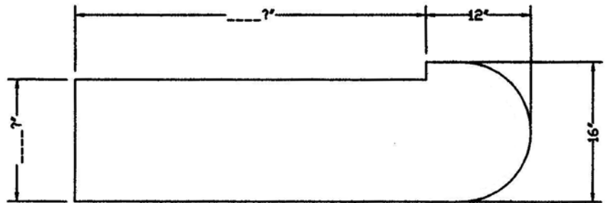
Half Round Starting Step (Right Hand Shown)
