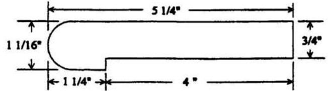
8590 Landing Tread 4'-12' Lengths 14'-16' Lengths
