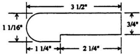
8090 Landing Tread 4'-12' Lengths 14'-16' Lengths
